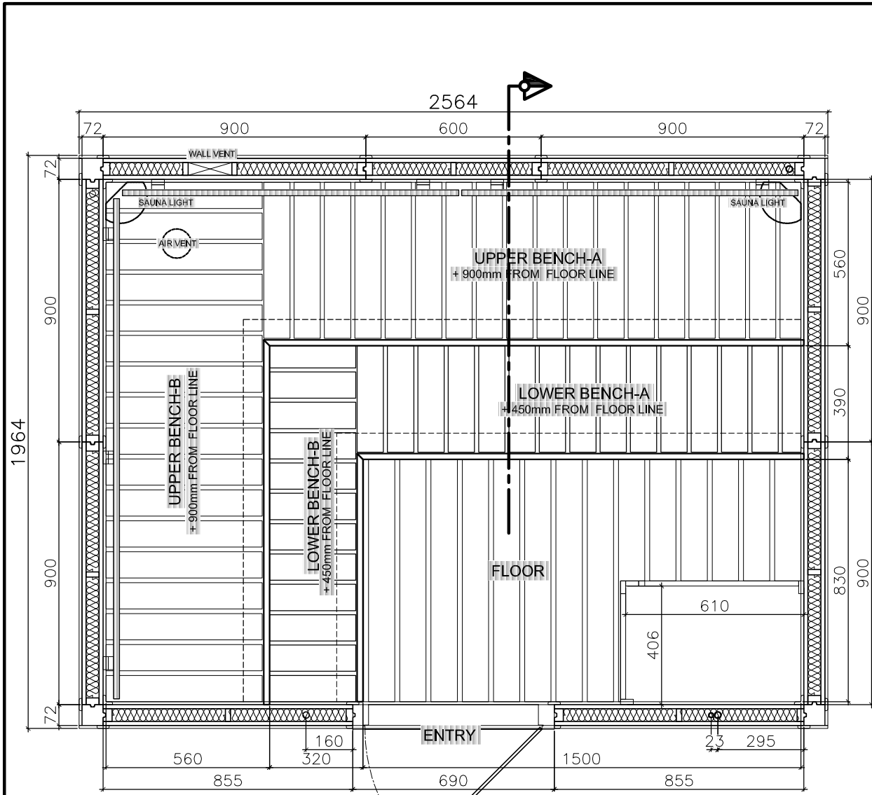
FLOOR PLAN FIT TO SCALE
