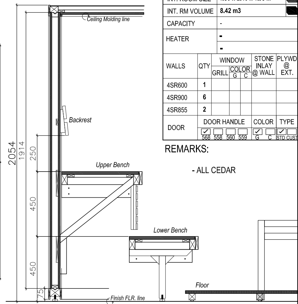
SECTION FIT TO SCALE
